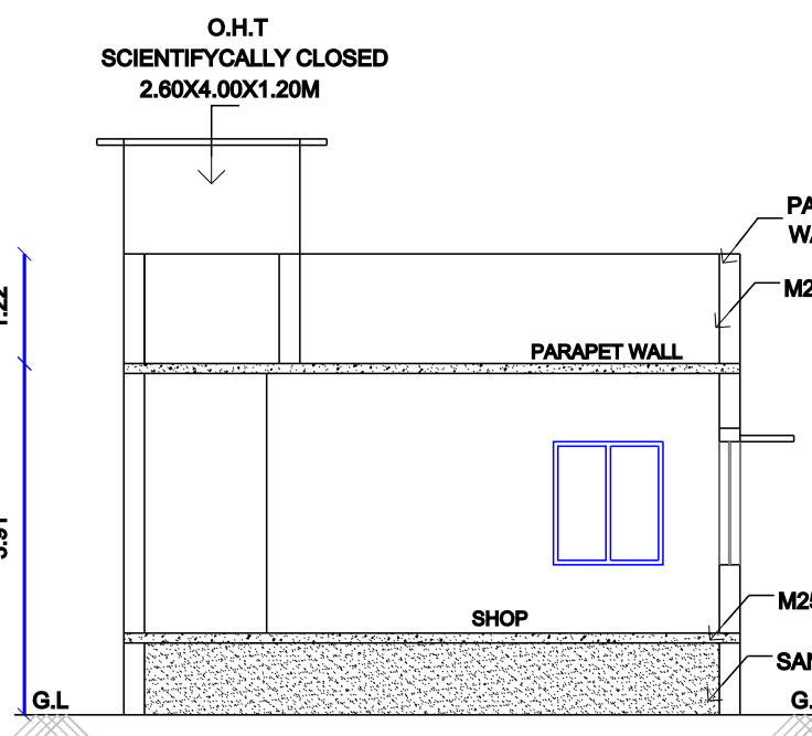
SECTION - AA (PROPOSED)
