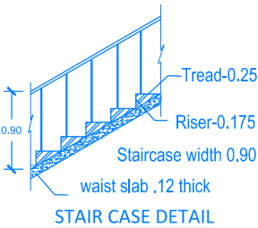
STAIR CASE DETAIL
