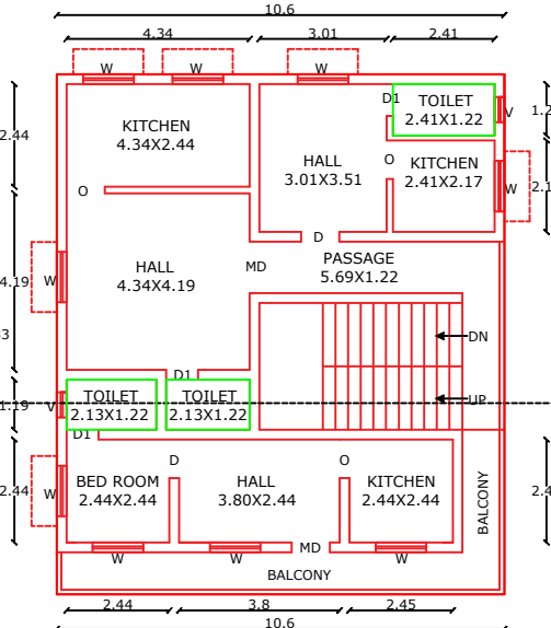
EXI.FIRST FLOOR PLAN
