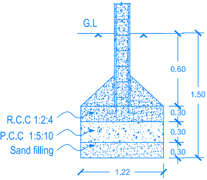
FOUNDATION DETAIL
