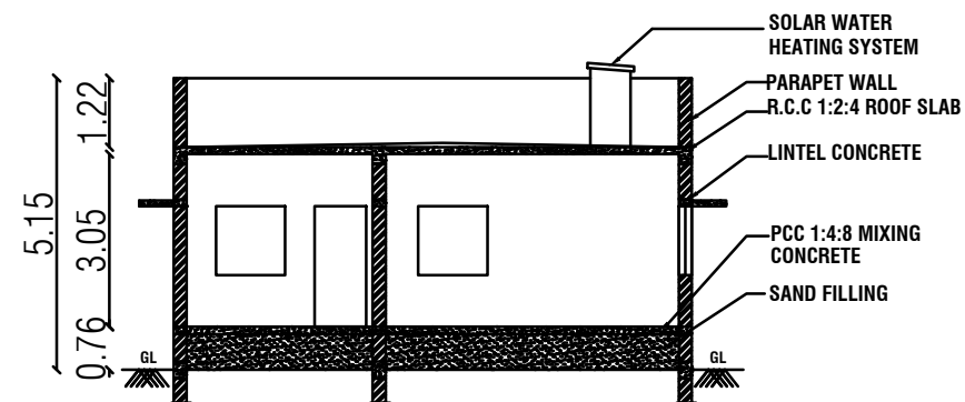
SECTION NO - "AB"
