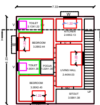
PRO.GROUND FLOOR PLAN
