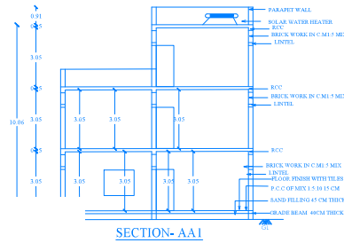
SECTION- AA1
