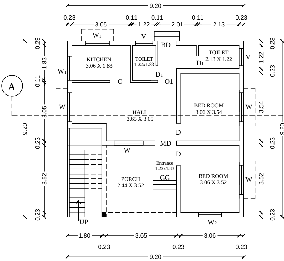
EXG - GROUND FLOOR PLAN
