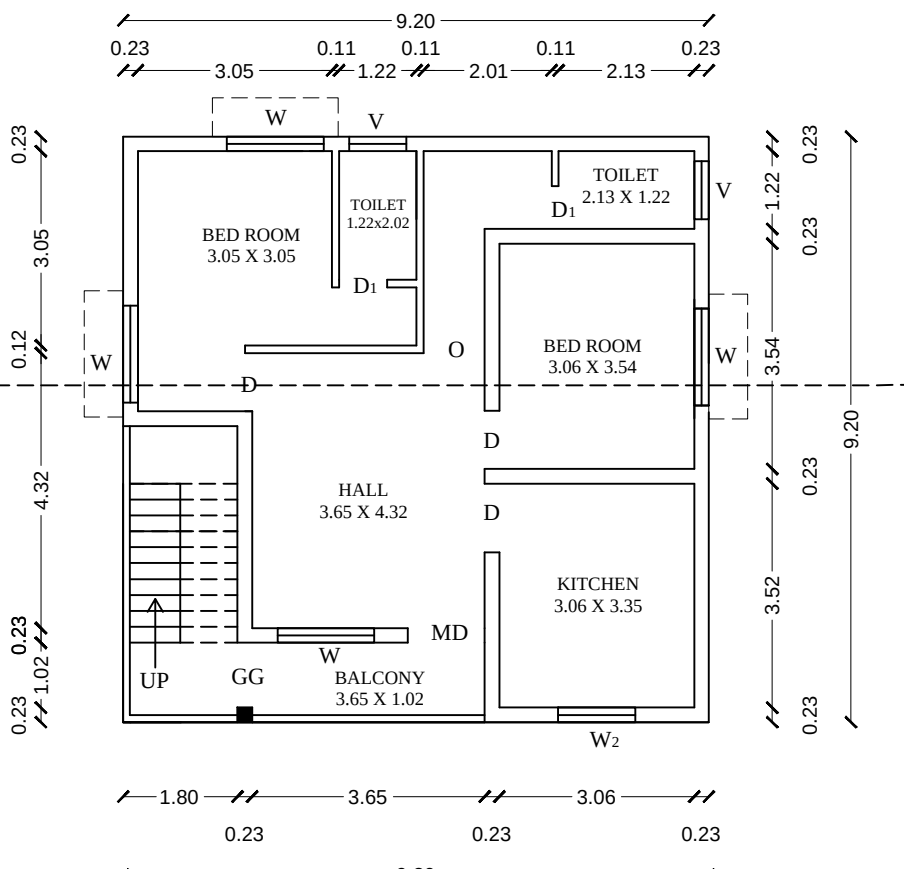
EXG - FIRST FLOOR PLAN
