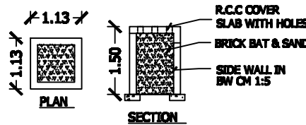
RAIN WATER HARVESTING PIT
