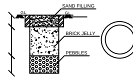
RAIN WATER HARVESTING SYSYTEM
