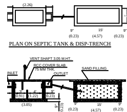
SECTION ON SEPTIC TANK & DISP-TRENCH
