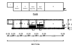
② SEWAGE TREATMENT PLANT DETAILS As Per G.O 158, dated 16.10.2002
