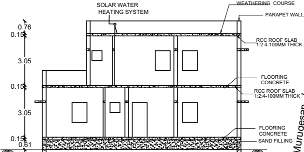
SECTION NP
