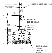
FOUNDATION DETAILS Scale 1:50
