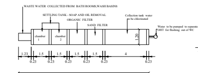
WASTE WATER RECYCLING SYSTEM
