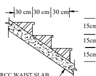
STAIR CASE STEPS SCALE 1:25
