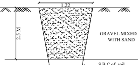
TRIAL PIT DETAILS
