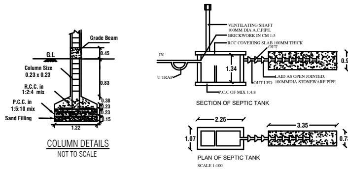
PLAN OF SEPTIC TANK SCALE 1:100
