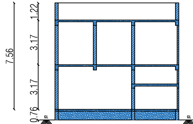
SECTION NO -"AB"
