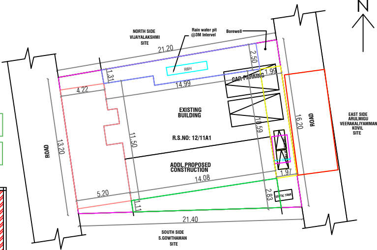
SITE PLAN
