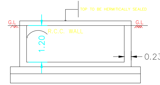
RWH_SECTION (SAMPLE)
