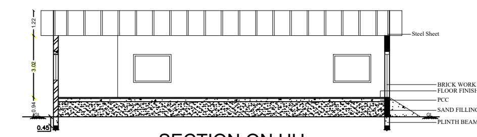
SECTION ON HH
