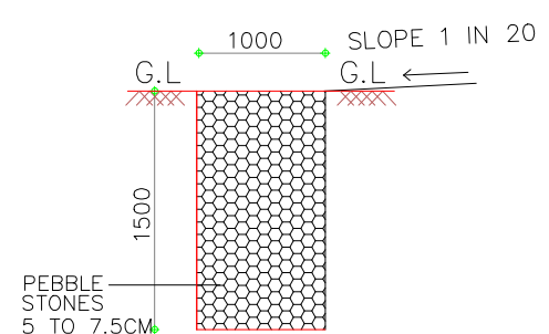
SECTION OF PEBBLE TRENCH
