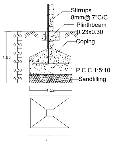
Foundation Details
