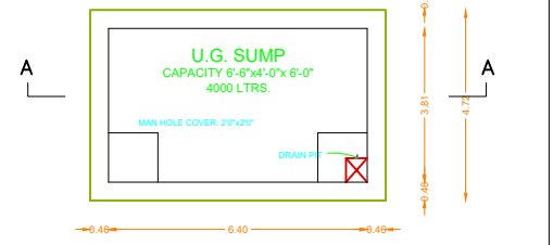
SUMP DETAIL SCALE 1"=4'0"
