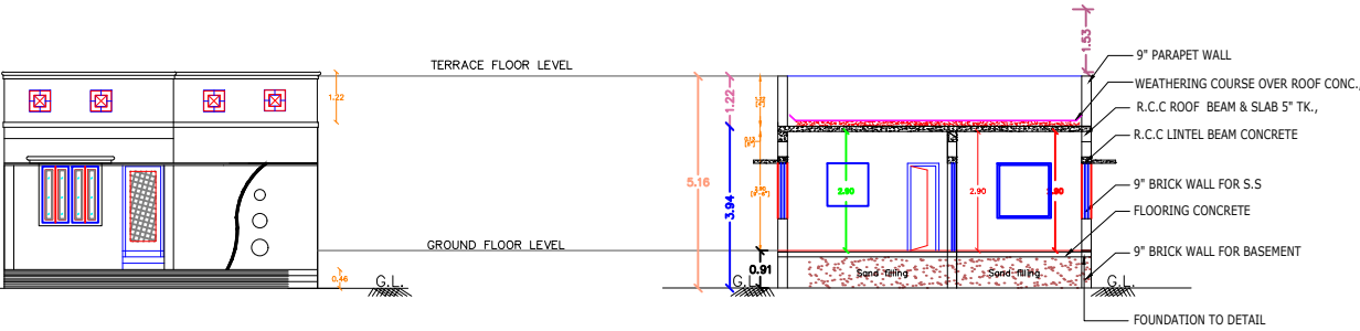
FRONT ELEVATION
