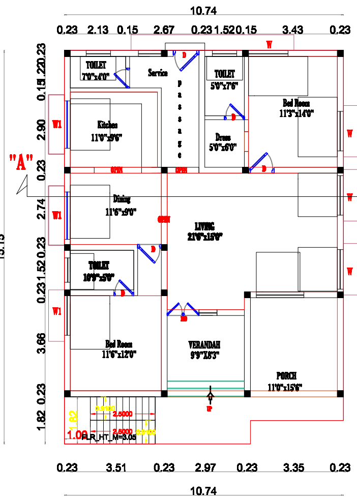
Pro.Ground Floor
