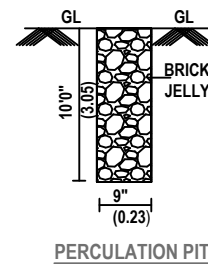
PERCOLATION PIT
