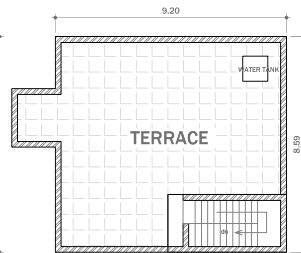
TERRACE PLAN
