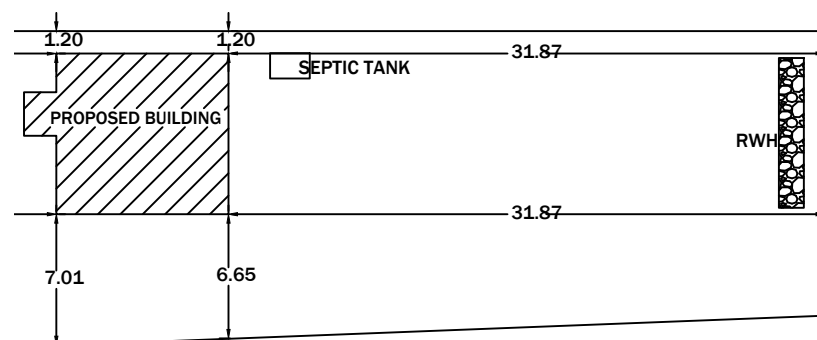
SITE PLAN
