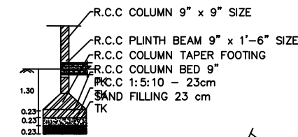
COLUMN DETAILS PLAN
