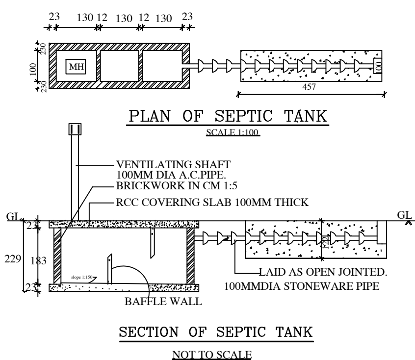
SECTION OF SEPTIC TANK NOT TO SCALE
