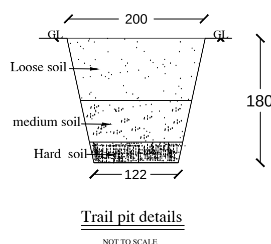
Trail pit details NOT TO SCALE
