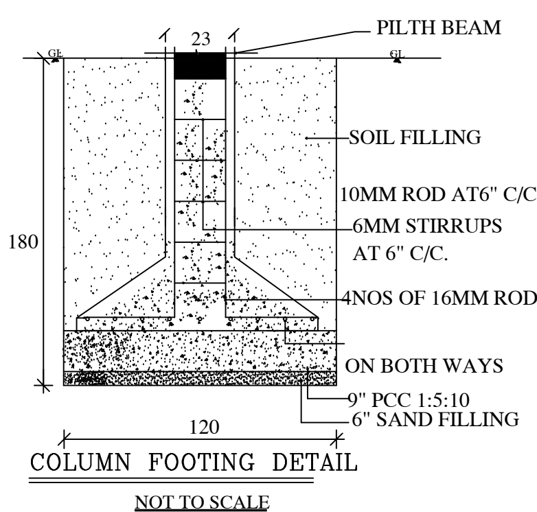
COLUMN FOOTING DETAIL NOT TO SCALE
