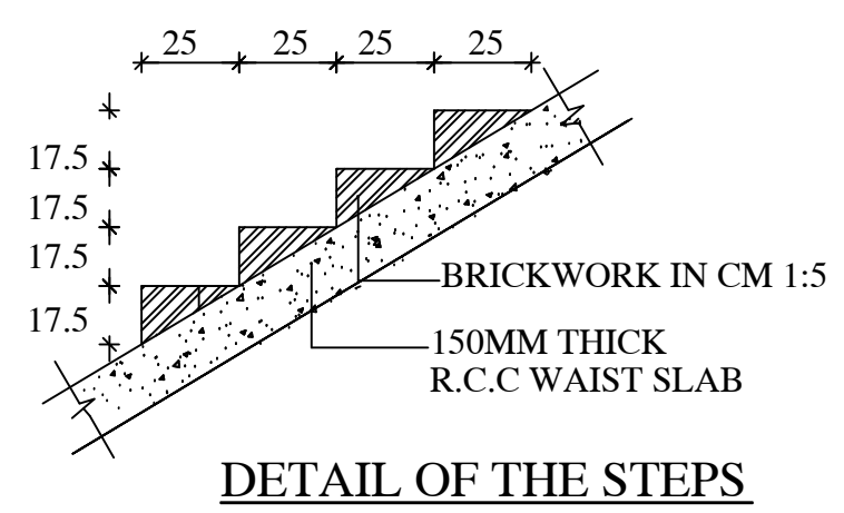
DETAIL OF THE STEPS SCALE 1:100
