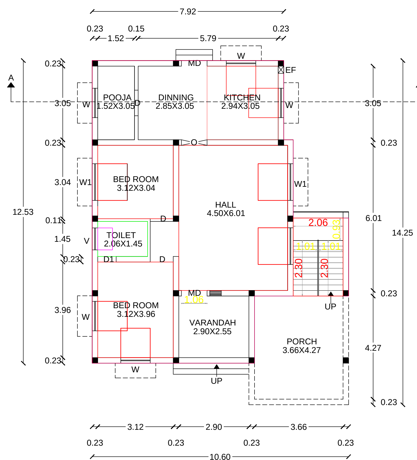
EXT.GROUND FLOOR BUILDING
