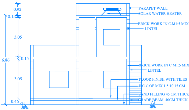
SECTION ON A-A1
