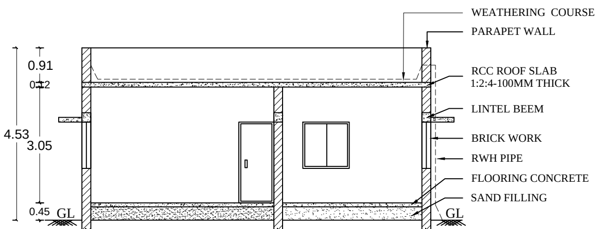
SECTION - XY
