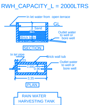
RAIN WATER HARVESTING TANK
