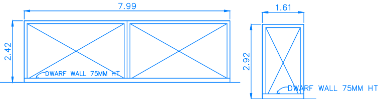
MAIN GATE
