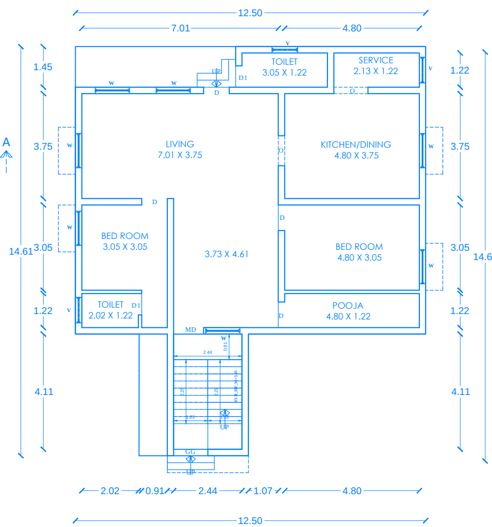
FLOOR PLAN
