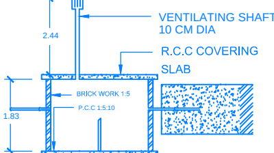
SEPTIC TANK DETAIL
