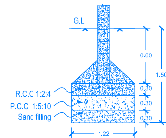
FOUNDATION DETAIL
