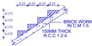
STAIRCASE DETAILS NOT TO SCALE
