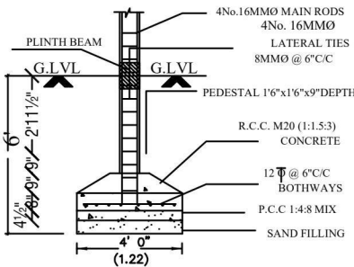
FOUNDATION DETAIL
