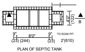
PLAN OF SEPTIC TANK
