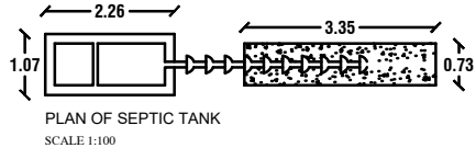
PLAN OF SEPTIC TANK SCALE 1:100
