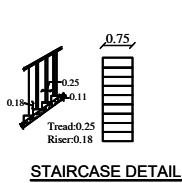
STAIRCASE DETAIL
