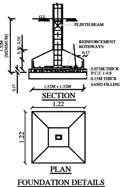
FOUNDATION DETAILS
