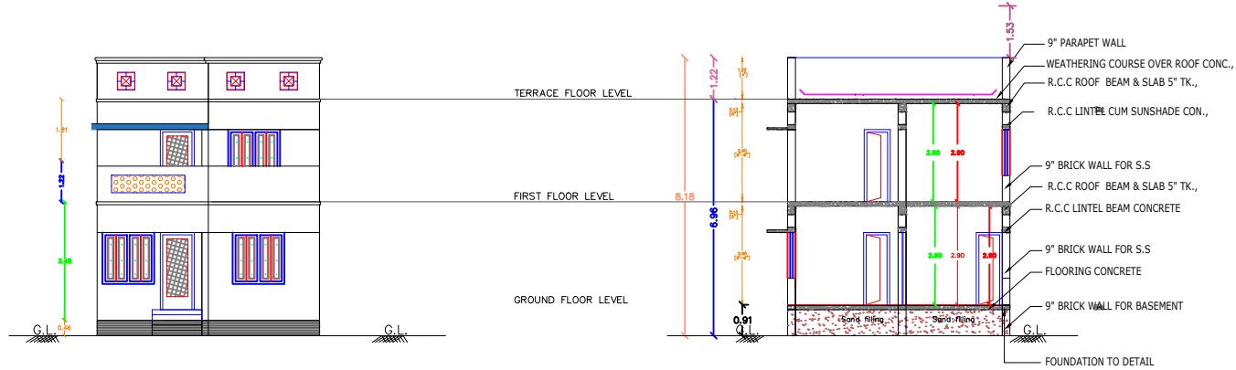
FRONT ELEVATION
