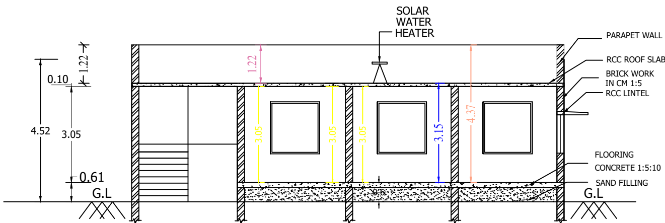
SECTION ON XX'
