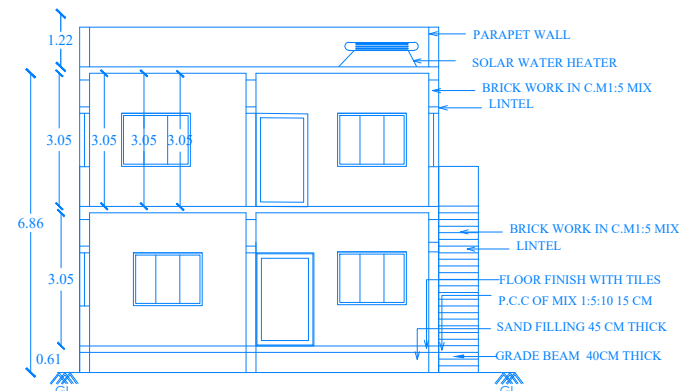
SECTION- AA1
