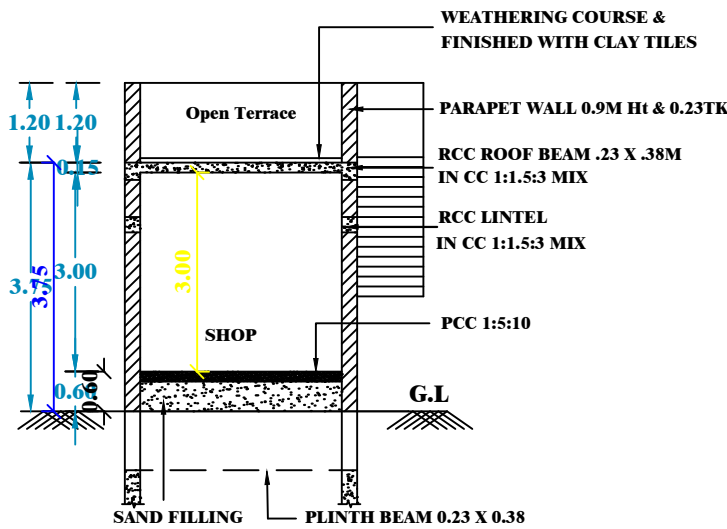
SECTION-XX
