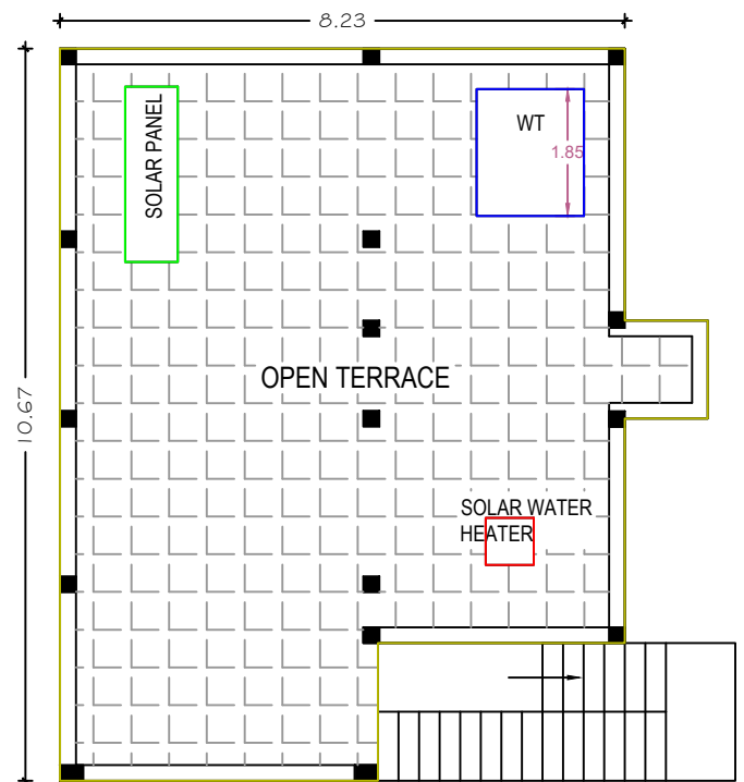
TERRACE PLAN
