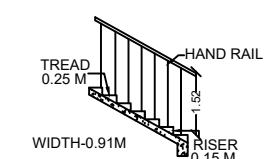
STAIRCASE DETAILS
