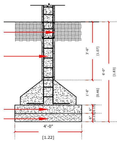
COLUMN FOUNDATION RCC COLUMN 0.23 x 0.30
