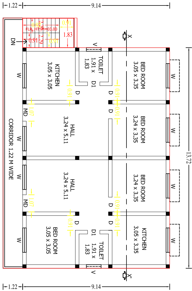
EXT. FIRST FLOOR PLAN
