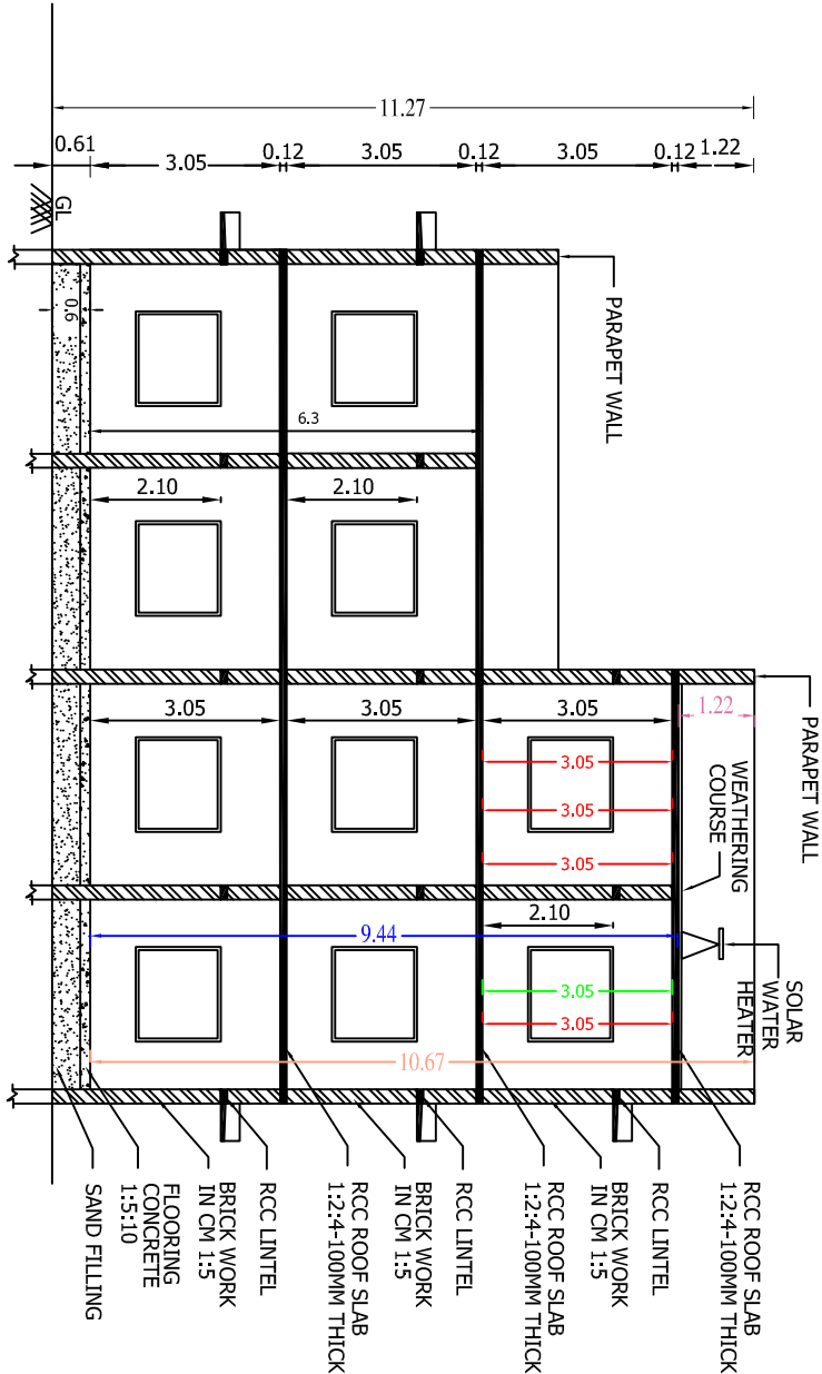
SECTION ON XX'
