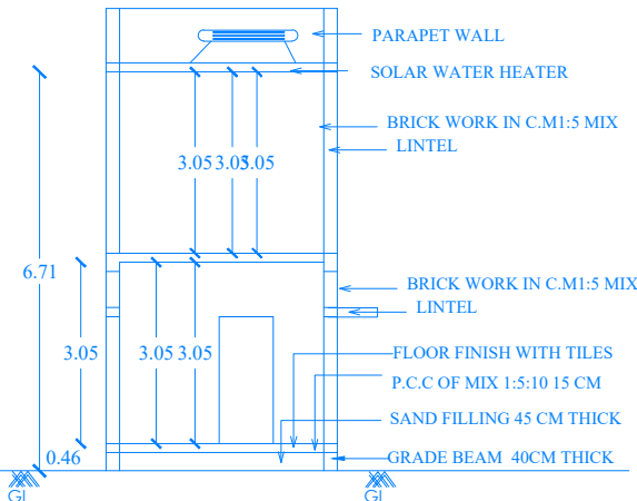
SECTION- AA1
