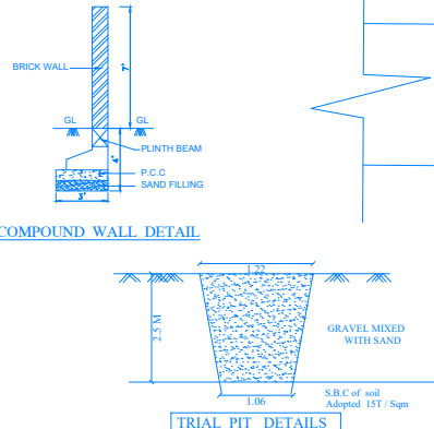
TRIAL PIT DETAILS
