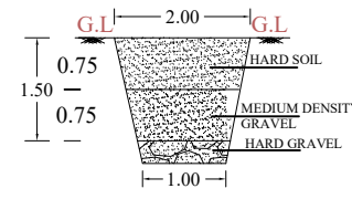
TRIAL PIT
