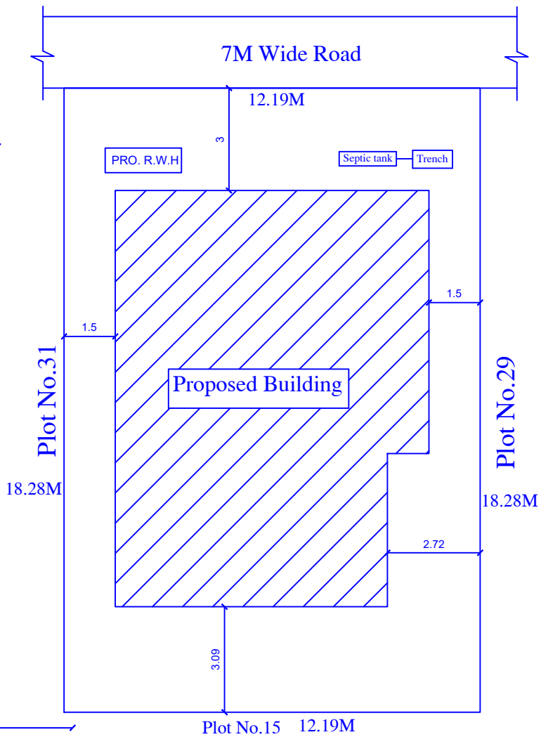
SITE PLAN
