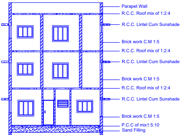
SECTION ON RS
