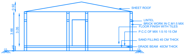
SECTION-AB
