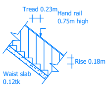
STAIR DETAILS
