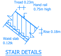
STAIR DETAILS
