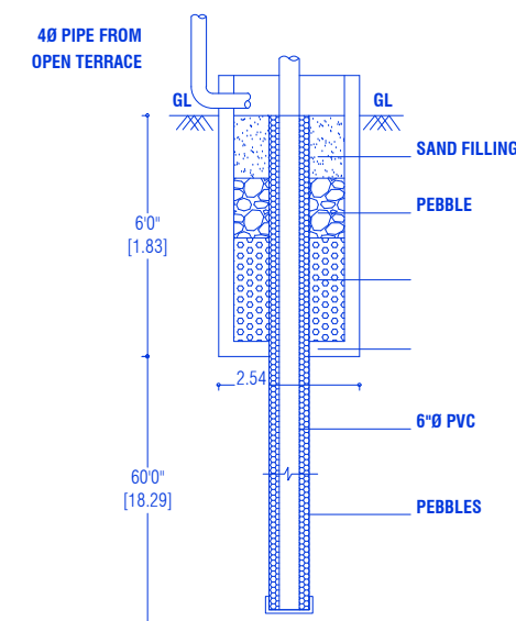
Section of Rain water Harvesting
