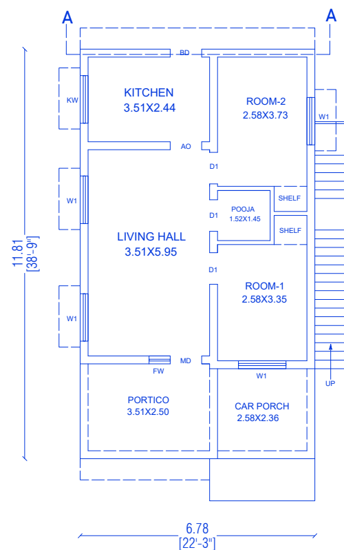
PRO-GROUND FLOOR
