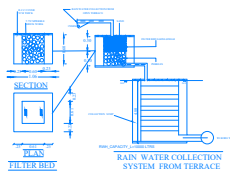
RAIN WATER COLLECTION SYSTEM FROM TERRACE
