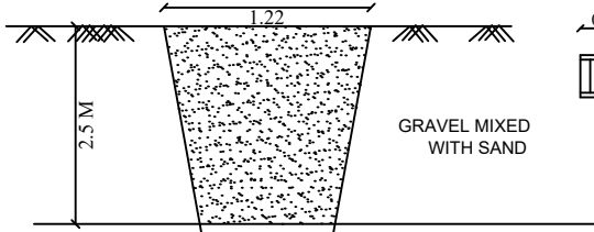
TRIAL PIT DETAILS
