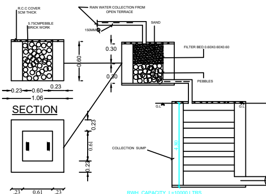
RAIN WATER COLLECTION SYSTEM FROM TERRACE
