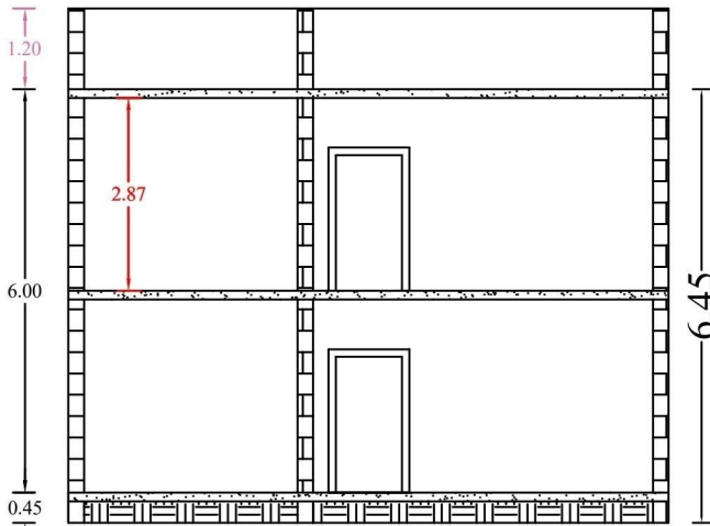
SECTION XX-XX
