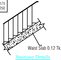
Staircase Details
