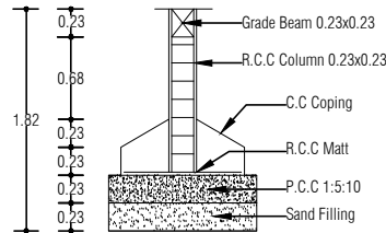
Foundation Detail
