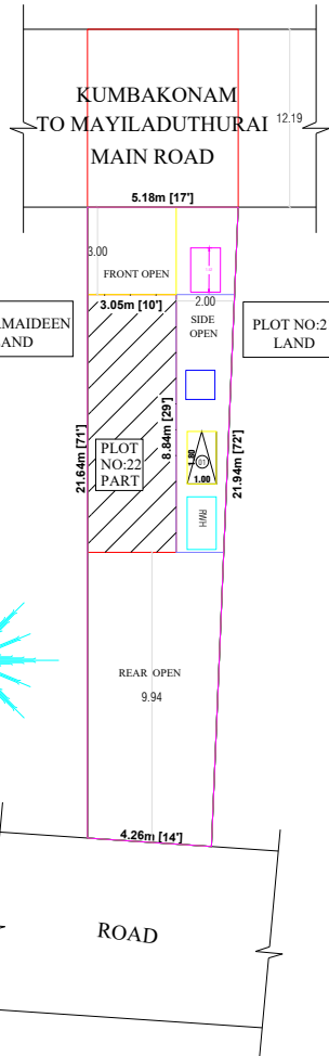
SITE PLAN
