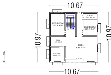
PRO.GROUND FLOOR PLAN
