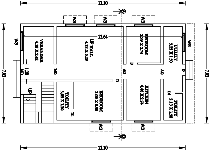
EXT. GROUND FLOOR PLAN
