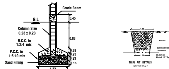
COLUMN DETAILS NOT TO SCALE
