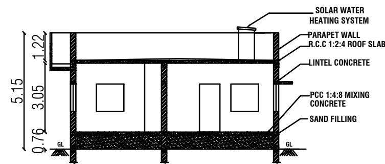
SECTION NO -"AB"
