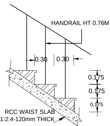
STAIR CASE STEPS SCALE 1:25
