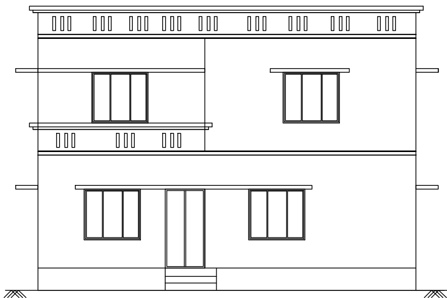
FRONT ELEVATION
