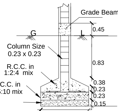
COLUMN DETAILS NOT TO SCALE
